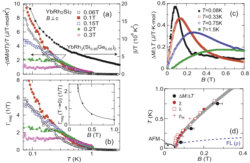
Figure 3. (a) Temperature derivative of the magnetization as -(dM/dT)/T (left axis) and (b) magnetic Grüneisen ratio \Gamma_{\text{mag}} as a function of temperature (on logarithmic scales) for YbRh 2 Si 2 at different magnetic fields applied perpendicular to the c axis. Volume thermal expansion of YbRh 2 (Si 0.95 Ge 0.05 ) 2 as -\beta/T at zero field is shown for comparison in (a) (right axis). Inset in (b): field dependence of saturated \Gamma_{\text{mag}} , as extrapolated to T = 0 . The solid line indicates -G(B - B_c^{\text{fit}})^{-1} with G = -0.3 and B_c^{\text{fit}} = 0.065 T. (c) Change in magnetization divided by temperature increment, -\Delta M/\Delta T , versus magnetic field for YbRh 2 Si 2 at T = 0.08 K (black), 0.33 K (red), 0.75 K (blue) and 1.5 K (green). (d) Temperature–field phase diagram including peak positions in -\Delta M/\Delta T and T^*(B) line (grey line) from transport and thermodynamic properties (red symbols). The solid black and the dashed blue lines represent the AF phase boundary and the NFL–LFL crossover, respectively (reproduced with permission from [19]. Copyright 2009 by the American Physical Society).
