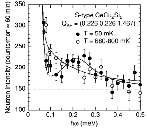
Figure 2. Energy scans (neutron intensity S = S_{ela} + S_{qe/ine,mag} versus energy transfer \hbar\omega ) in S-type CeCu_2Si_2 at Q = Q_{AF} = (0.226 \ 0.226 \ 1.467) in the superconducting state at T = 0.05 K, B = 0 . For comparison the magnetic response at Q_{AF} in the normal state at T = (0.68-0.8) K > T_c = 0.6 K, B = 0 is also plotted. The solid lines represent fits to the data comprised of the incoherent and coherent elastic contributions, and the inelastic or quasielastic magnetic signal at Q_{AF} , convoluted with the resolution. The magnetic signal is modelled by a Lorentzian line. The dashed line represents the constant background as determined at negative energy transfers (reproduced with permission from [18]. Copyright 2007, Elsevier).
